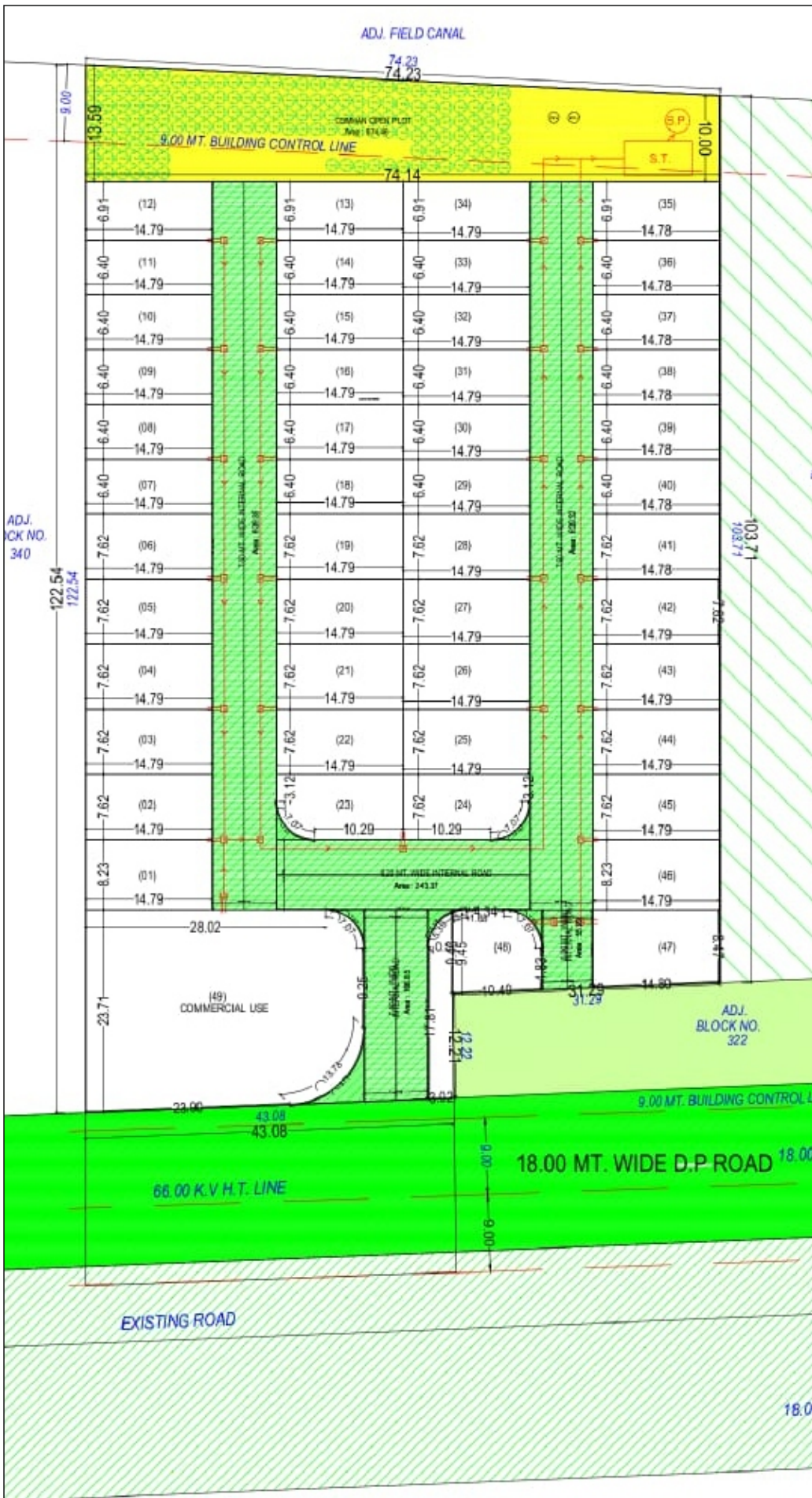
LAYOUT PLAN (Scale - 1:400)
